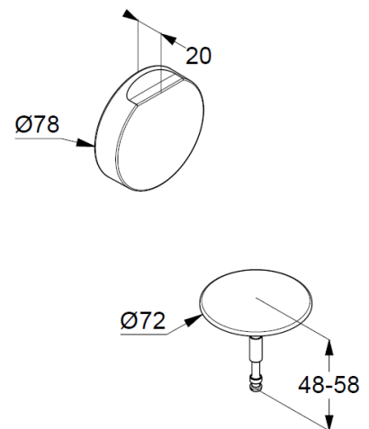
Dimensional drawing
