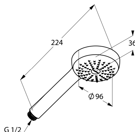
Dimensional drawing
