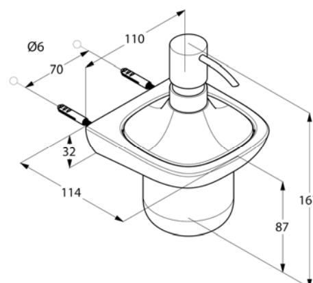
Dimensional drawing
