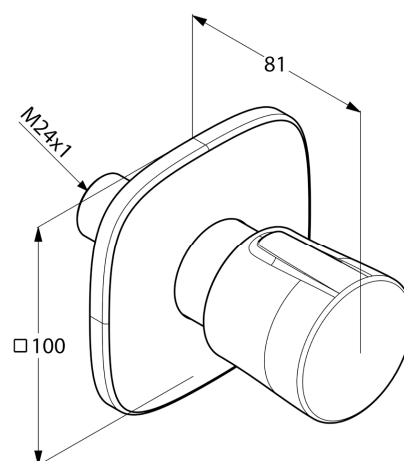
Dimensional drawing I
