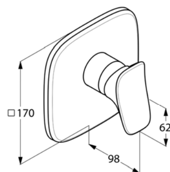
Dimensional drawing
