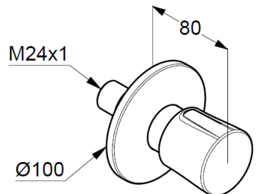
Dimensional drawing
