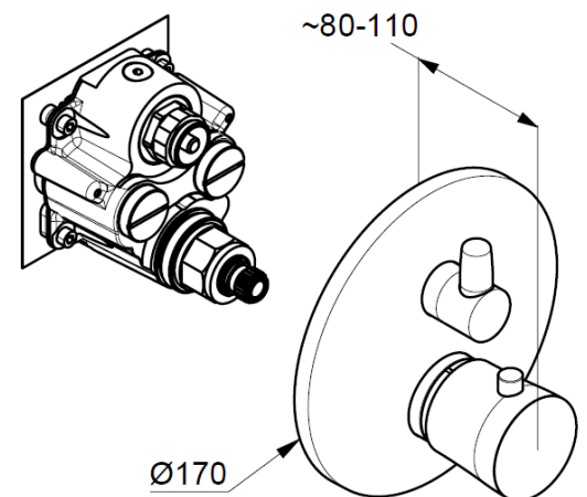
Dimensional drawing
