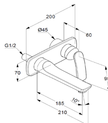
Dimensional drawing
