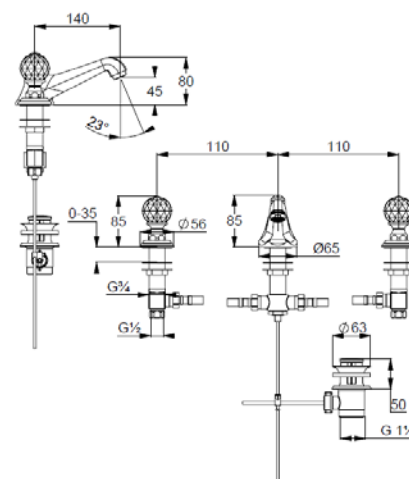
Dimensional drawing
