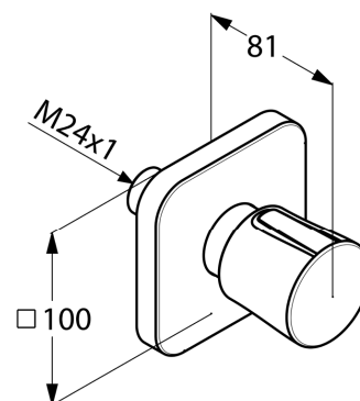
Dimensional drawing I
