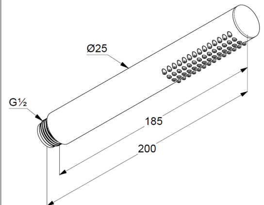
Dimensional drawing
