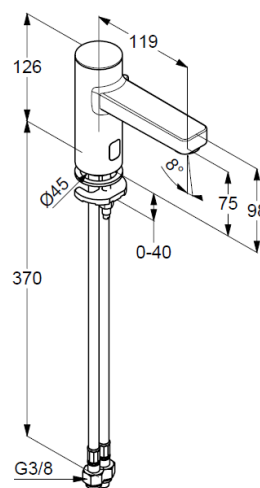
Dimensional drawing
