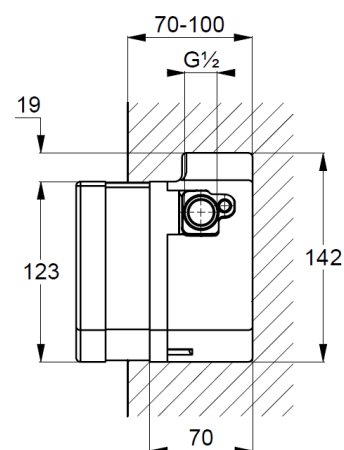
Dimensional drawing
