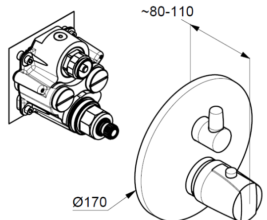
Dimensional drawing
