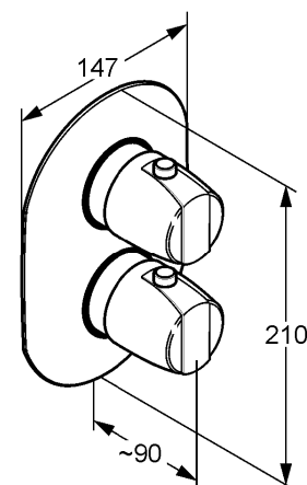
Dimensional drawing I
