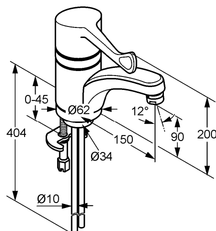
Dimensional drawing
