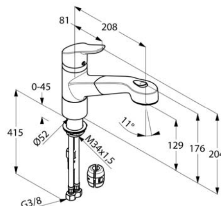
Dimensional drawing
