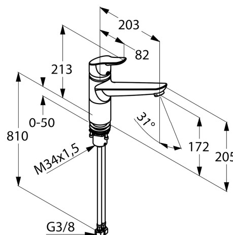
Dimensional drawing
