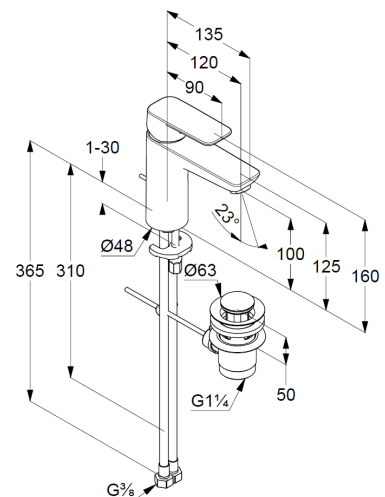
Dimensional drawing
